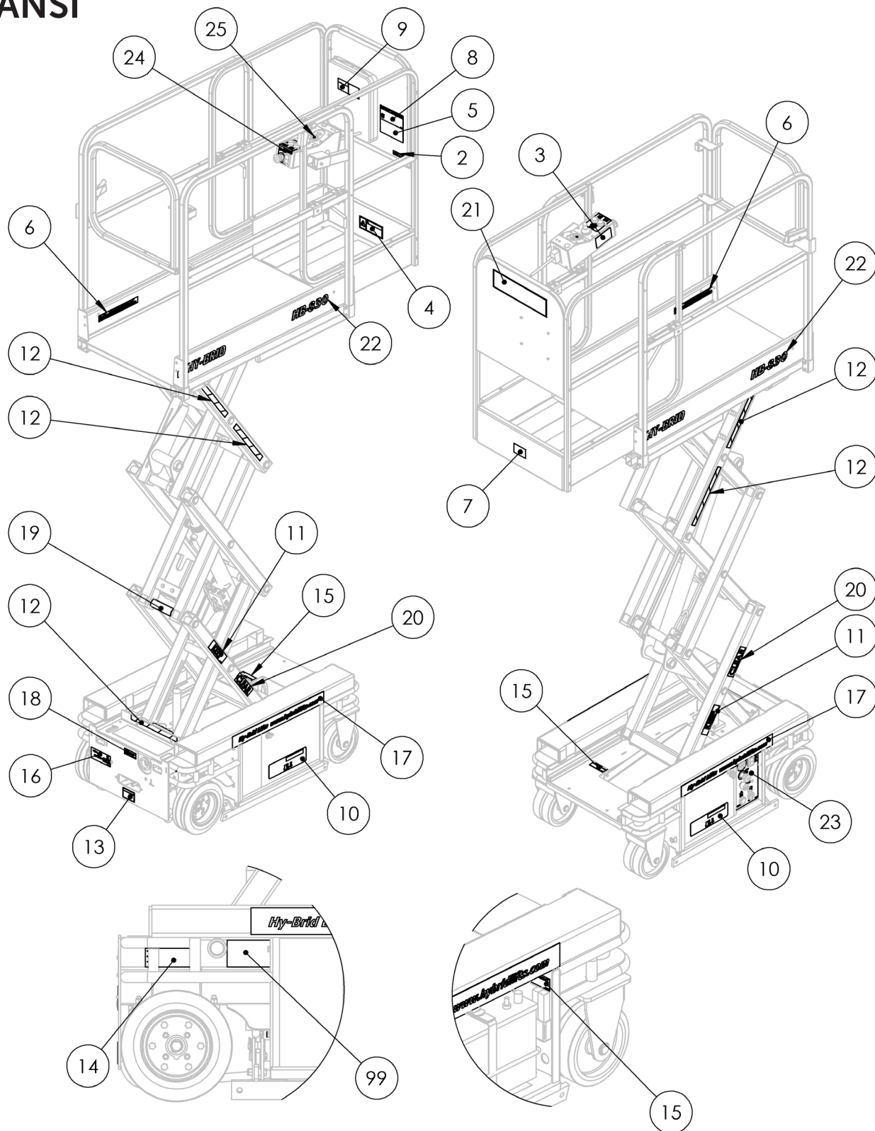
FIGURE 1: Decal Locations - HB-830
