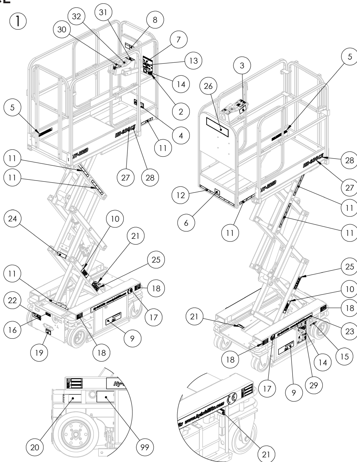
FIGURE 2: Decal Locations - HB-830CE
