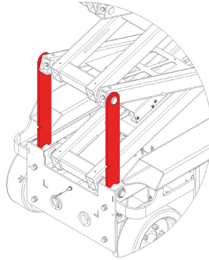
FIGURE 7: Maintenance Lock In Use
