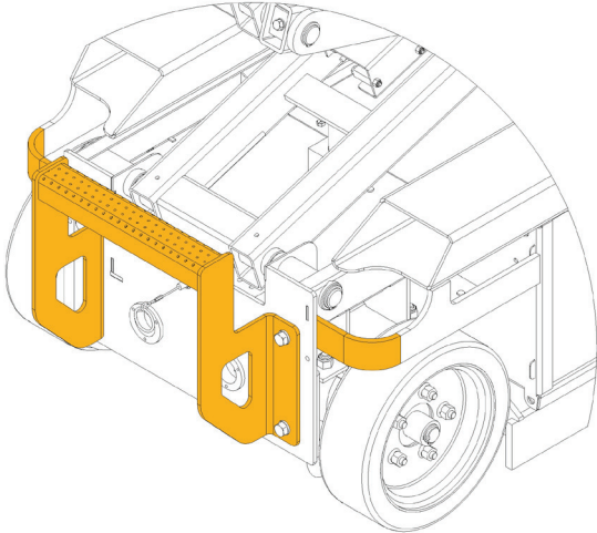
FIGURE 11: Tie-Down Points, Rear
