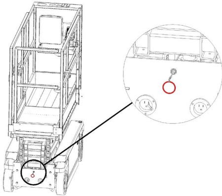
FIGURE 4: Auxiliary Lowering
