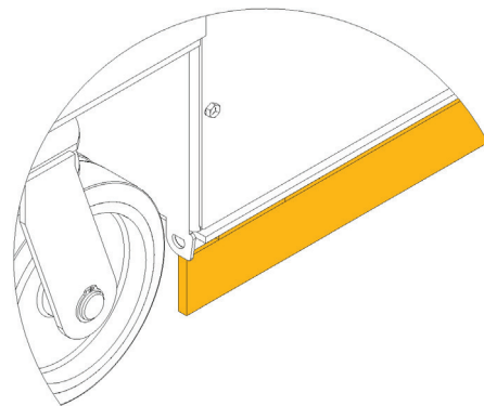
FIGURE 3: Pothole Guard
