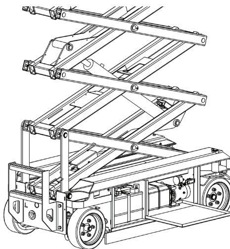
FIGURE 26: LeakGuard™ Location
