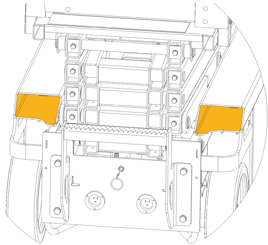
FIGURE 13: Fork Pockets
