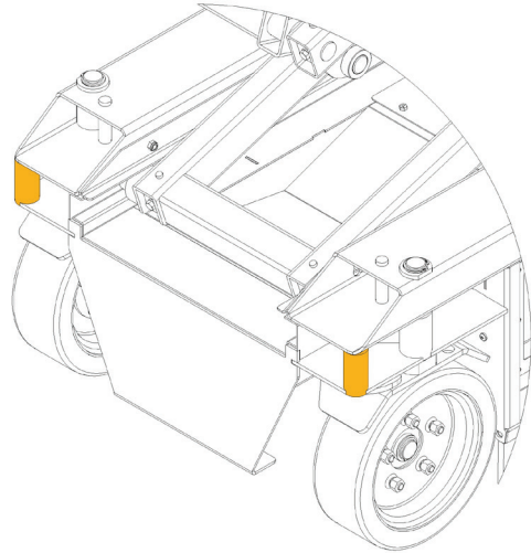
FIGURE 12: Tie-Down Points, Front
