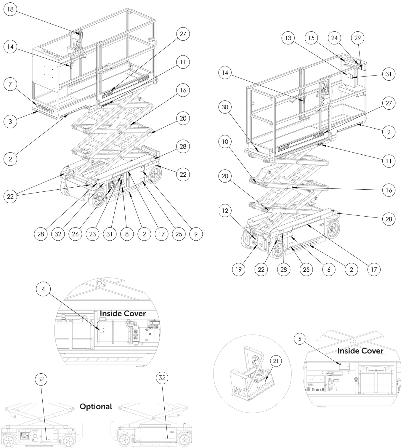
FIGURE 9: PS-1430 Decal Locations
