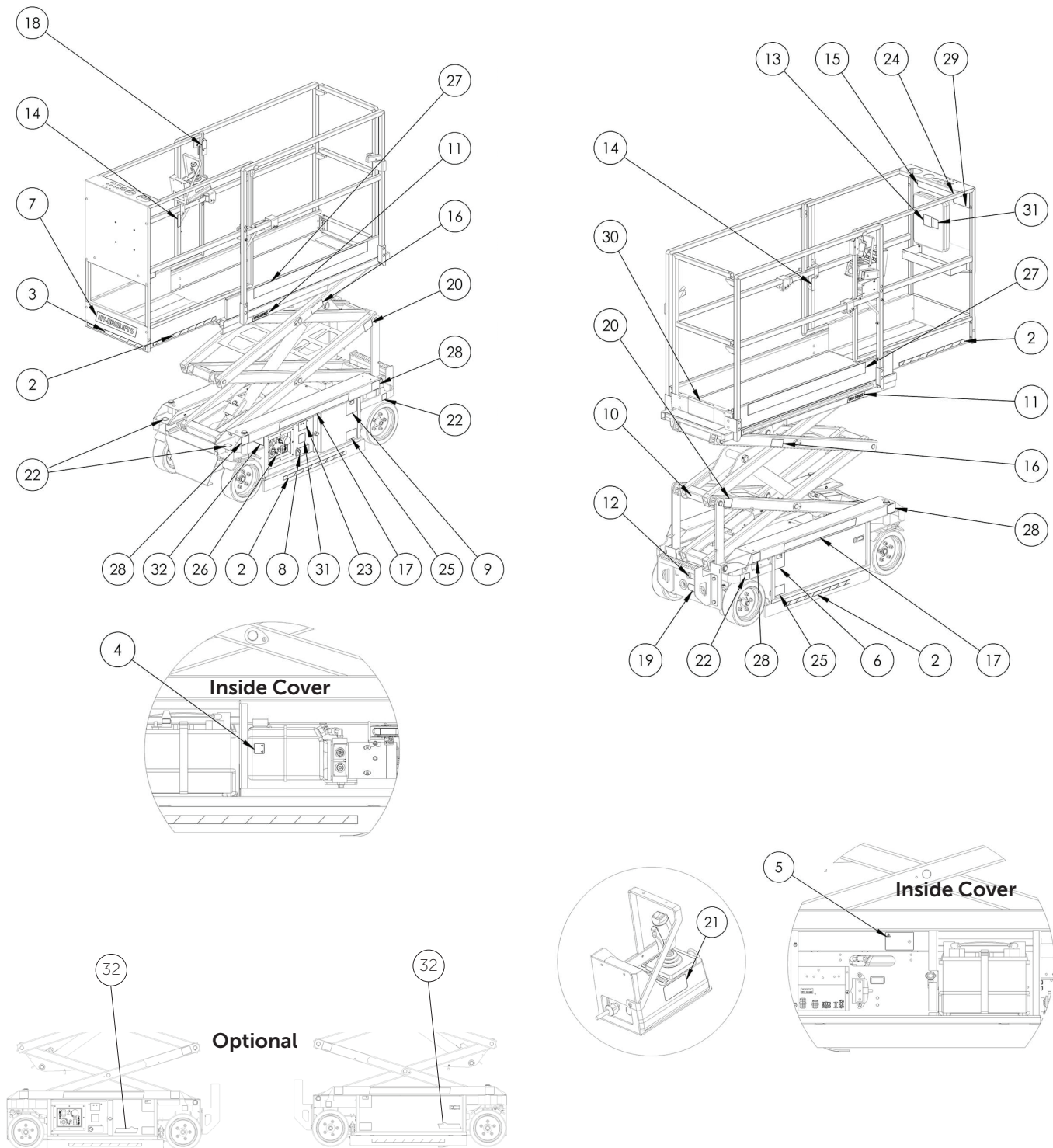
FIGURE 8: PS-1030 Decal Locations
