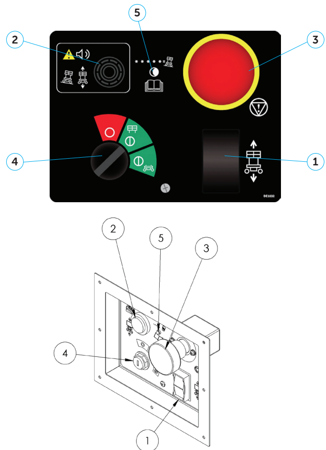
FIGURE 15: Base Controls
