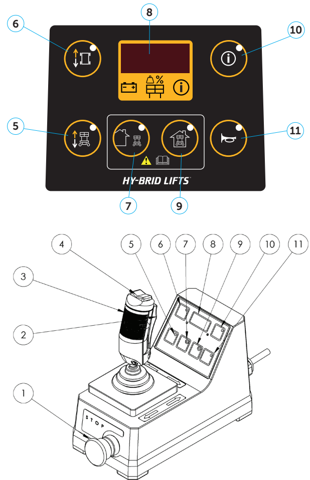
FIGURE 16: Platform Controls Style 1
