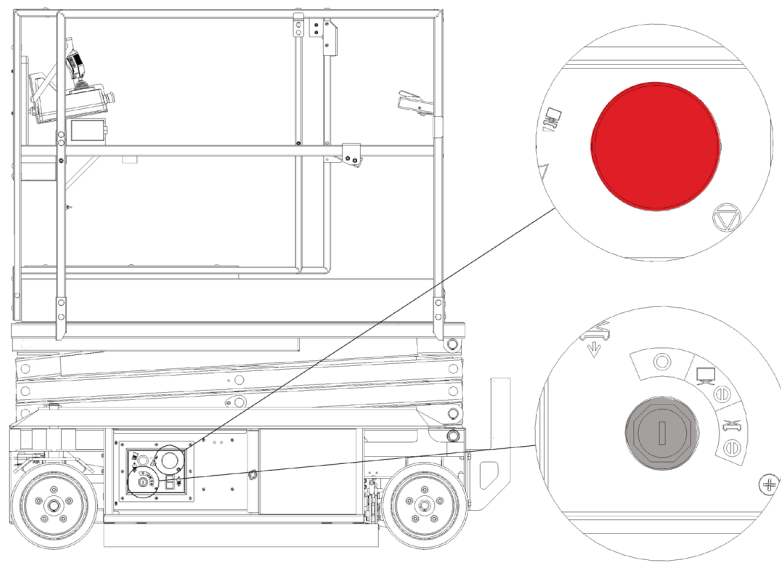
FIGURE 19: Master Power and Key Switch
