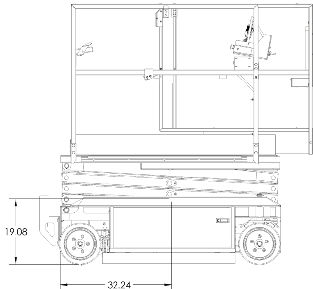
FIGURE 14: Center of Gravity
