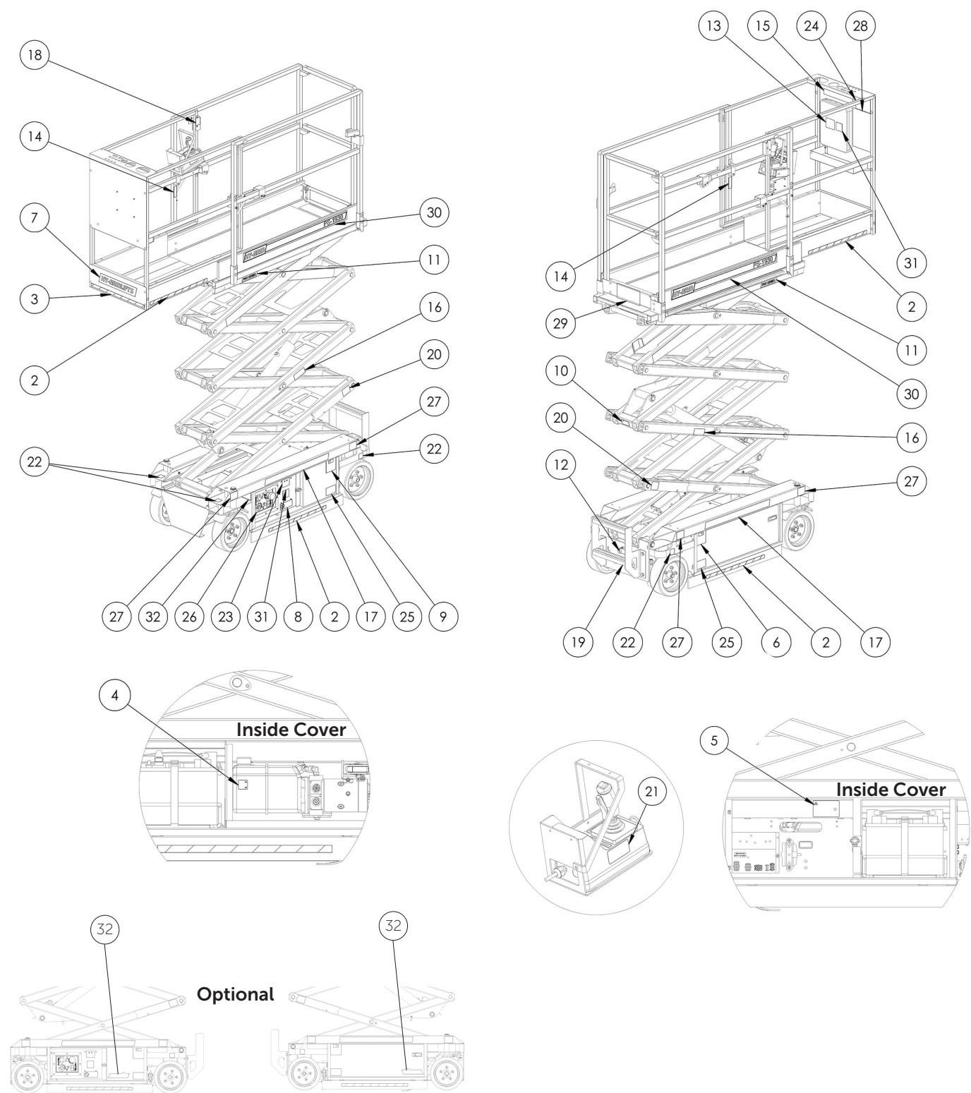
FIGURE 10: PS-1930 Decal Locations
